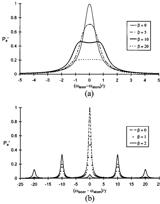
FIG. 2. Effect of micromotion on the spectrum of P_e (excited state population). We plot P_e' = P_e[\hbar\gamma/(2\mathcal{P}|E_0|)]^2 for various values of \beta . For both graphs, we assume that the ion is driven below the saturation limit. (a) \Omega/\gamma = 0.1 . For \beta = 10 , heating occurs in the regions <0.6 < (\omega_{\text{laser}} - \omega_{\text{atom}})/\gamma < 0 and (\omega_{\text{laser}} - \omega_{\text{atom}})/\gamma > 0.6 . (b) \Omega/\gamma = 10 . For \beta > 0 , heating can occur when the laser frequency is tuned near, but above the center of, any of the sideband frequencies.
