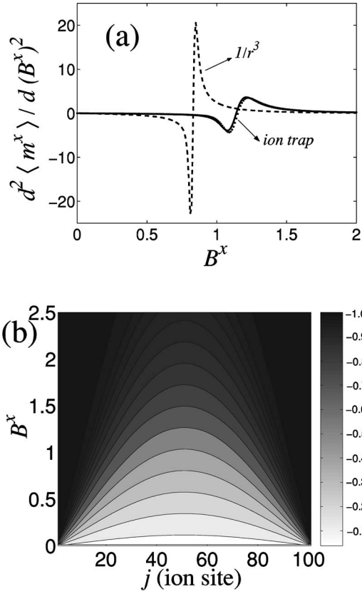
FIG. 2. (a) Second derivative of m^x as a function of B^x in ion trap Ising models ( N=100 ions). Dashed line, 1/r^3 Ising model; solid line, average over the 20 central ions in a linear trap Ising model; dotted line, central ( j=50 ) ion in a linear trap Ising model (solid and dotted lines are almost on top of each other). (b) Contour plot of \langle \sigma_j^z \rangle^2 on the plane of the coordinate j and the magnetic field B^x .
