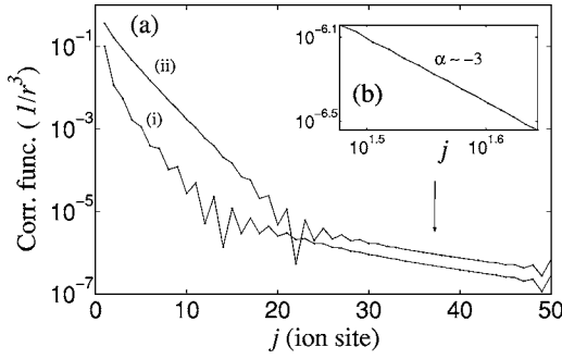
FIG. 4. (a) Absolute value of correlations |C_{j_0 j_0+j}^{\alpha\alpha}| between the central ion ( j_0=50 ) and the rest of a chain with N=100 ions, in the case of the 1/r^3 Ising model. (i) C_{j_0 j_0+j}^{xx} , B^x=0.72 < B_c^x ; (ii) C_{j_0 j_0+j}^{zz} , B^x=1.32 > B_c^x . (b) Zoom of the long-range tail of C^{zz} , which follows an algebraic decay with an exponent \alpha=-3 .
