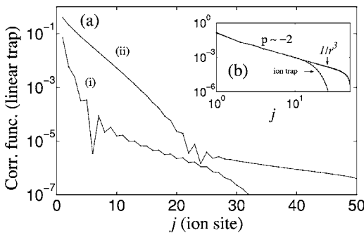
FIG. 5. (a) Absolute value of correlations |C_{j_0 j_0+j}^{\alpha\alpha}| between the central ion ( j_0=50 ) and the rest of a chain with N=100 ions, in the case of the linear trap Ising model. (i) C_{j_0 j_0+j}^{xx} , B^x=0.89 < B_c^x ; (ii) C_{j_0 j_0+j}^{zz} , B^x=1.72 > B_c^x . (b) Plot of C_{j_0 j_0+j}^{xx} for both 1/r^3 and linear ion trap models, exactly at the critical point B^x=B_c^x . At intermediate distances, both curves are well fitted by a power-law decay C_{j_0 j_0+j}^{xx} \propto |j|^p , with p=-2 , the same critical exponent that corresponds to the NN Ising model.
