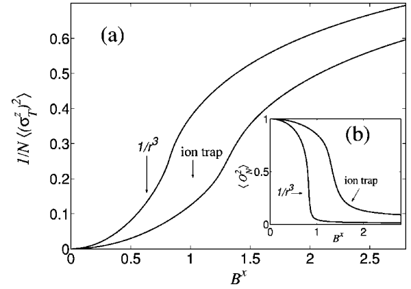
FIG. 3. (a) Fluctuation of the longitudinal effective magnetization, and (b) Néel order parameter. In both plots we consider the 1/r^3 Ising model and the central region (20 ions) of the linear trap Ising model.
