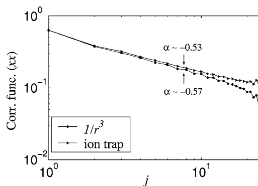
FIG. 10. Correlation C_{j_0, j_0+j}^{xx} between the central ion j_0=26 and the rest of the chain in the critical region as a function of ion separation j . C_{j_0, j_0+j}^{xx} is well fitted by a power-law decay with the exponents \alpha shown in the figure.
