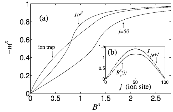
FIG. 1. (a) Evolution of the averaged effective transverse magnetization in 1/r^3 and linear trap Ising models ( N=100 ions). We also plot \langle \sigma_j^x \rangle in the case of the central ion ( j=50 ) in a linear trap. (b) Local strength of the Ising interaction in a linear ion trap, and local value of the critical field.
