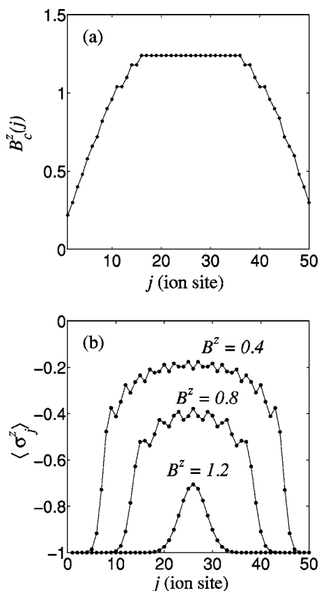
FIG. 9. (a) Local critical field calculated from the evolution of \langle \sigma_j^z \rangle in the linear trap XY model. (b) Spatial dependence of \langle \sigma_j^z \rangle in a linear trap XY model with different values of B^z .
