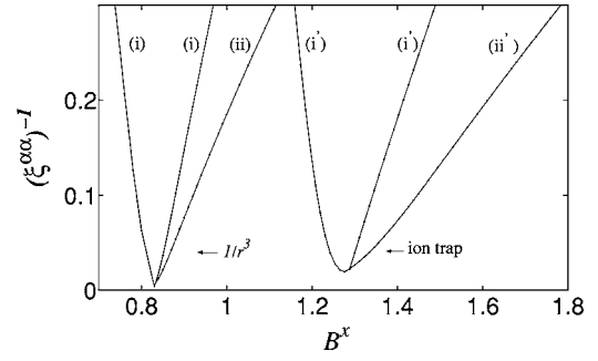
FIG. 6. Correlation lengths (\xi^{\alpha\alpha})^{-1} as a function of B^x in both 1/r^3 and linear ion trap models. (i), (i') curves correspond to (\xi^{xx})^{-1} , whereas (ii), (ii'), (ii) correspond to (\xi^{zz})^{-1} . \xi^{zz} is not shown in the antiferromagnetic phase because C_{i,j}^{zz} tends to a constant value in the absence of symmetry breaking.
