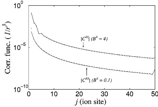
FIG. 7. (a) Absolute value of correlations |C_{j_0 j_0+j}^{\alpha\alpha}| ( j_0=50 , N=100 ions) in the case of the 1/r^3 Ising model. Points, numerical results from the DMRG calculations; solid line, calculation with the HP transformation.
