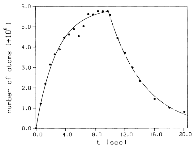
FIG. 2. Total fluorescence from the magnetically trapped atoms as a function of time. A new bunch was loaded every 0.65 s, for the first 10 s. The dot-dashed line is an exponential decay fit to the data, with 4.9 s 1/e time. The y axis has been calibrated to indicate the total number of trapped atoms.
