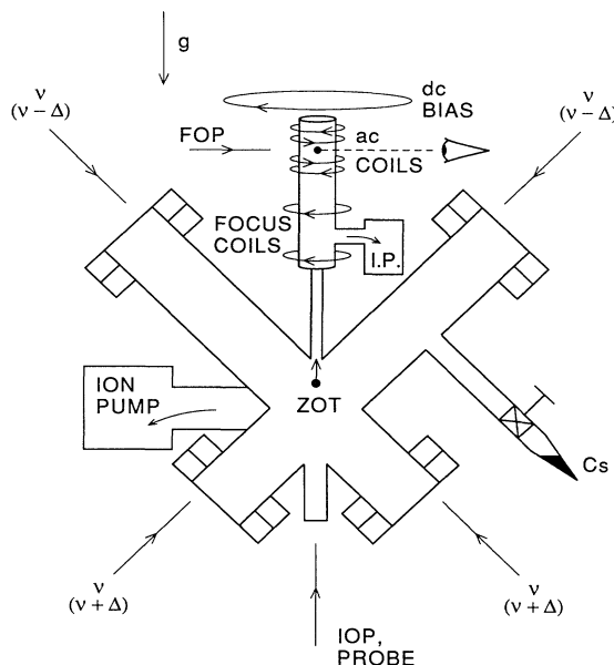
FIG. 1. Schematic of the apparatus, showing the upper and lower vacuum chambers, the configuration of key trapping and focusing coils, the paths of the initial optical pumping (IOP) and final optical pumping (FOP) laser beams, and the paths of four of the six laser beams defining the Zeeman-shift optical trap (ZOT) and the molasses. Frequencies of the molasses laser beams during the launch are shown in parentheses. Not shown are the paths of two horizontal laser beams which are perpendicular to the plane of the paper at the ZOT, the magnetic coils for tuning the optical trap, and a variety of shim magnetic coils.
